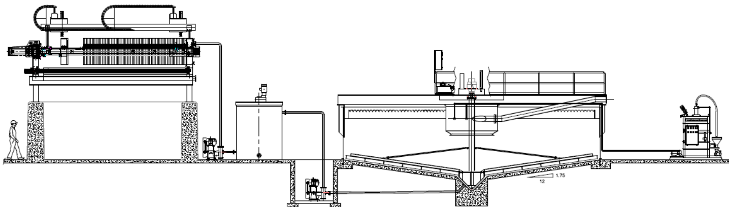
Top: Westpro 90ft diameter Clarifier in Canada Middle: Westpro 26ft diameter Clarifier in Canada Bottom: Typical Fines Removal System elevation view
